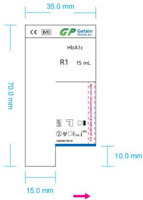
Reagent 1 Tube label (R1)
