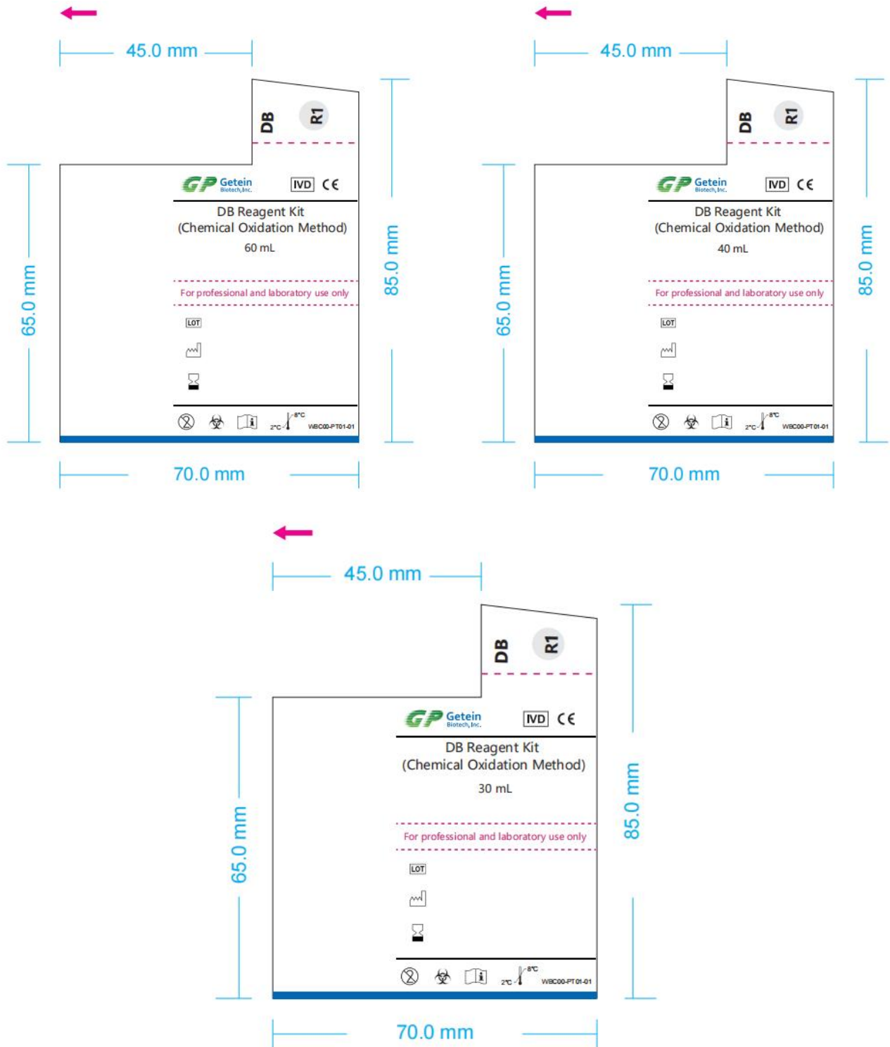
Reagent 1 Tube label (R1)
